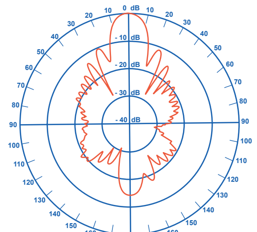
Plan E
